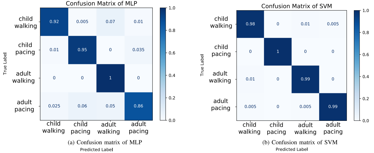
Fig. 7. Confusion matrices.
